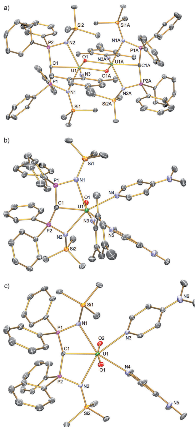
Figure 1. Single-crystal X-ray structures of a) [\{\text{U}(\text{BIPM}^{\text{TMS}})(\text{NMe})_2(\mu\text{-O})_2\}]_2 ( 4 ), b) [\text{U}(\text{BIPM}^{\text{TMS}})(\text{NMe})(\text{O})(\text{DMAP})_2] ( 5 ), and c) [\text{U}(\text{BIPM}^{\text{TMS}})(\text{O})_2(\text{DMAP})_2] ( 6 ). Displacement ellipsoids set at 40% probability. Hydrogen atoms, any lattice solvent, and minor disorder components are omitted for clarity. Selected bond lengths [Å]: 4 : U1–C1 2.408(3), U1–N1 2.408(3), U1–N2 2.374(3), U1–N3 1.943(3), U1–O1 1.953(2), U1–O1A 2.337(2); 5 : U1–C1 2.400(3), U1–N1 2.554(2), U1–N2 2.577(2), U1–N3 1.921(2), U1–N4 2.592(2), U1–N5 2.611(2), U1–O1 1.814(2); 6 : U1–C1 2.383(3), U1–N1 2.606(2), U1–N2 2.600(2), U1–N3 2.564(3), U1–N4 2.594(3), U1–O1 1.794(2), U1–O2 1.785(2).
